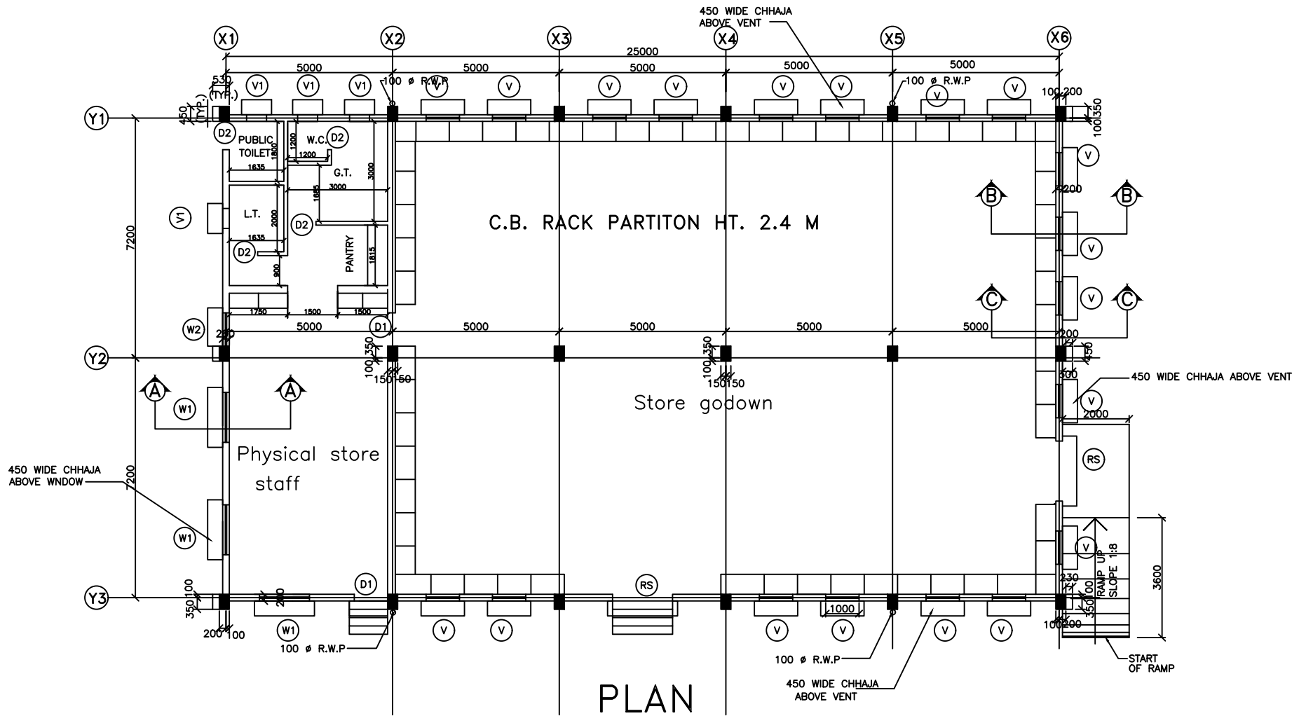
Sabarmati Divisional Store Plan
