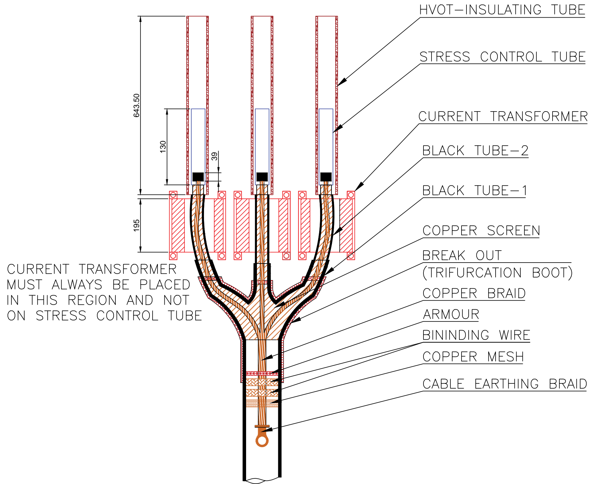
CABLE TERMINATION ARRANGEMENT
