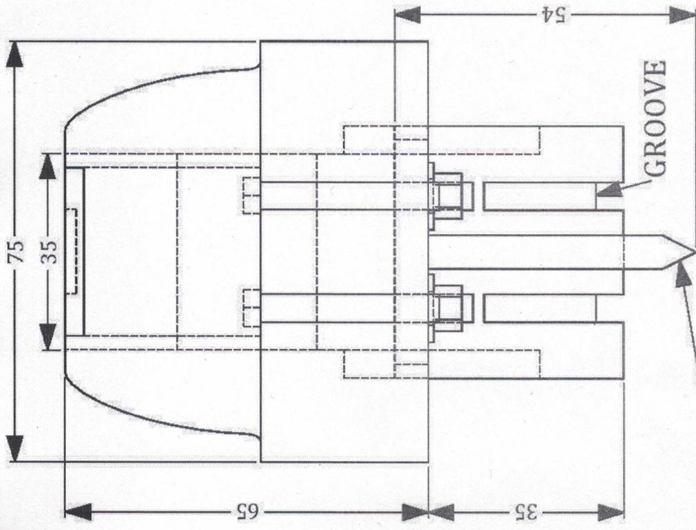
PART X SIDE VIEW
