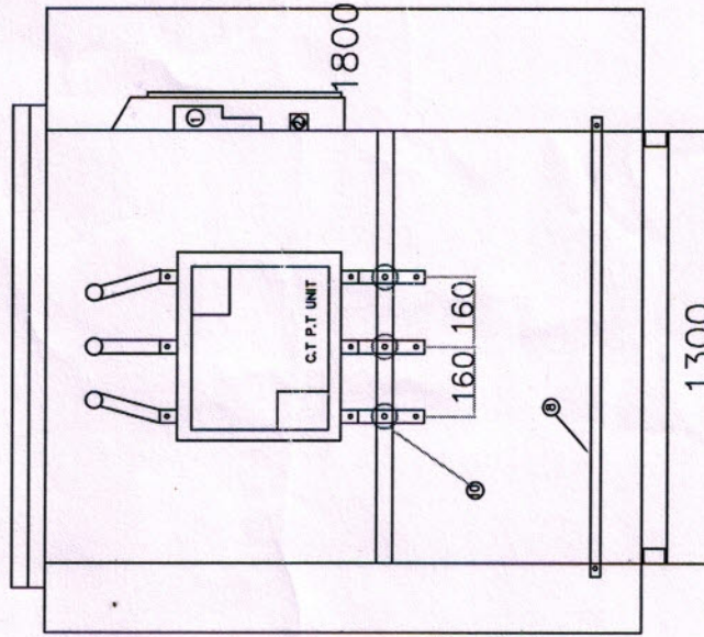
REAR VIEW DOOR OPENED
