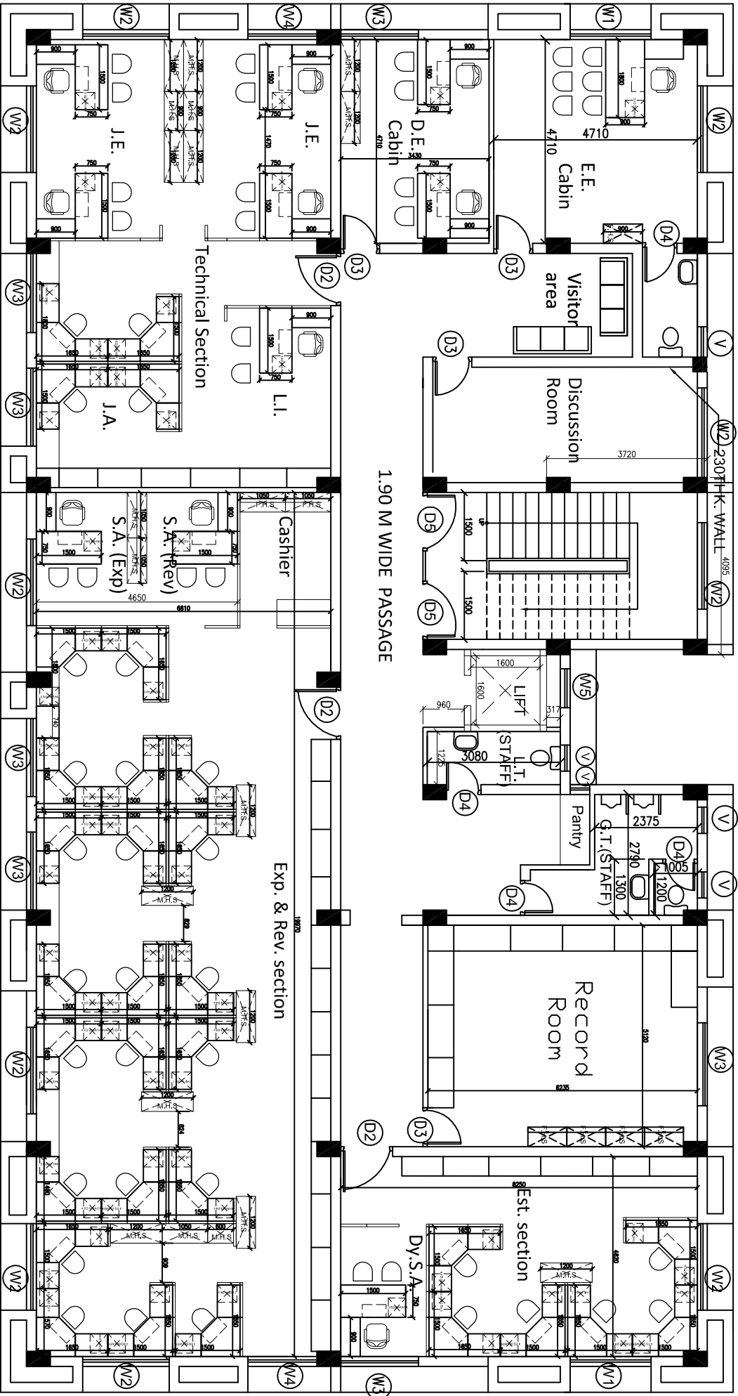
PROPOSED NEW ADMN. BLOCK (S.F.) BOPAL DIVISION OFFICE
