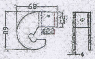
1. BOTTOM ASSEMBLY
