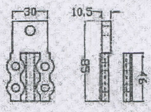
8. TERMINAL CONNECTOR
