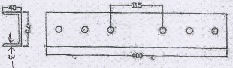
10. BASE CHANNEL
